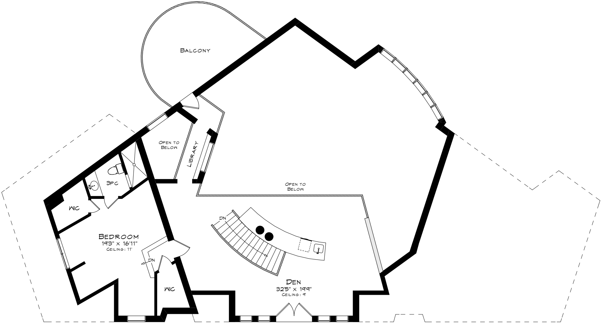
LOFT LEVEL PLAN 1,188 SQUARE FEET
